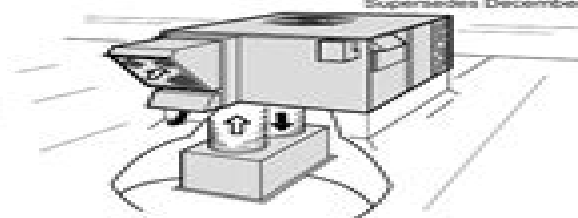
Rooftop Installation With Combination Supply and Return Air System
