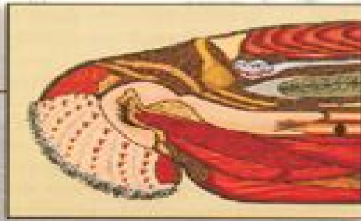
Figure 4c: Lamprey head.
