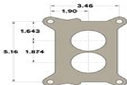
HOLLEY 2300 2-BBL
