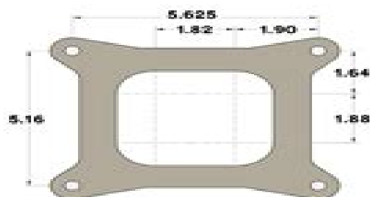
HOLLEY 4150/4160
