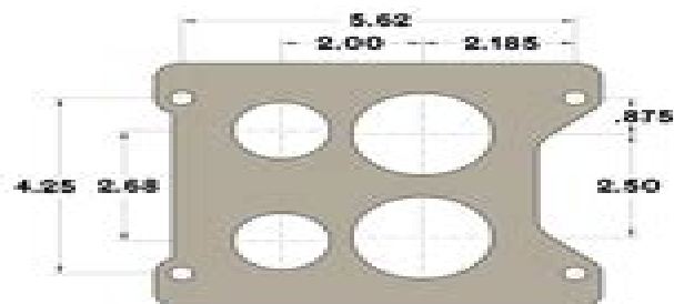
SPREADBORE (4165/4175)
