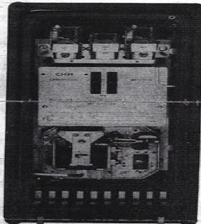
Type CMM41 relay in size 1 1/2 drawout case
