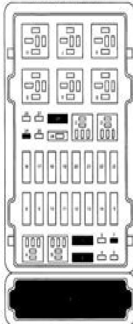
BATTERY JUNCTION BOX
