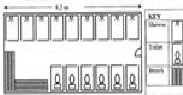
LAYOUT PLAN OF THE ABLUTION FACILITIES
