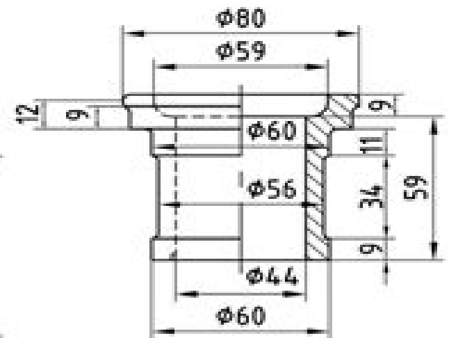
BUSH
